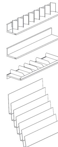
Multidrilled sides for adjustable shelves
